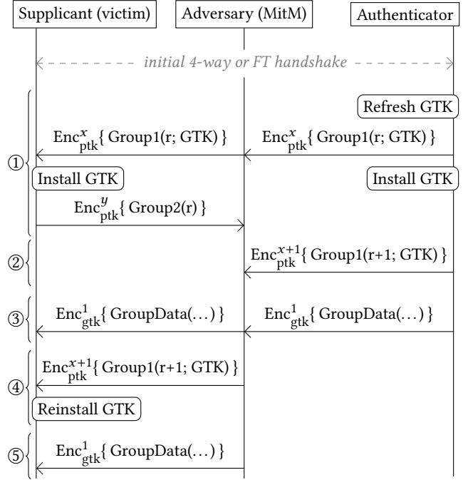
Figure 7: Key reinstallation attack against the group key handshake, when the authenticator (AP) immediately installs the GTK after sending a Group Message 1 to all clients.
